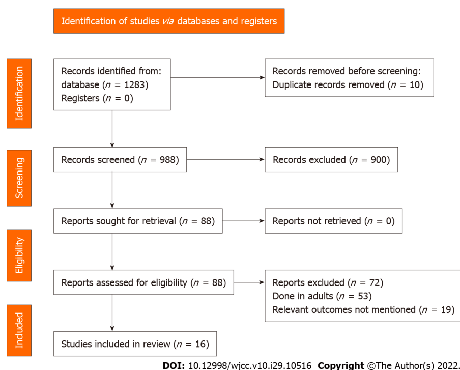
Figure 1 PRISMA flowchart.
